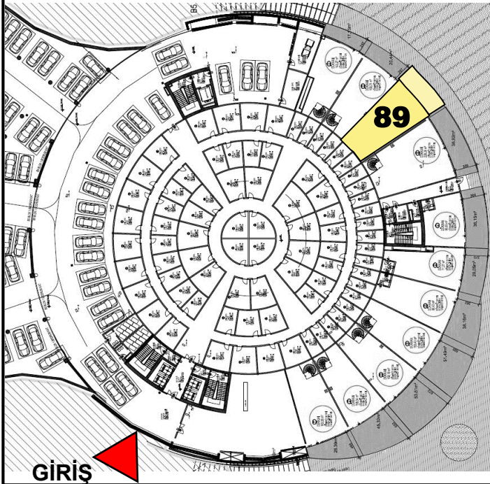
1. BODRUM KAT PLANI
